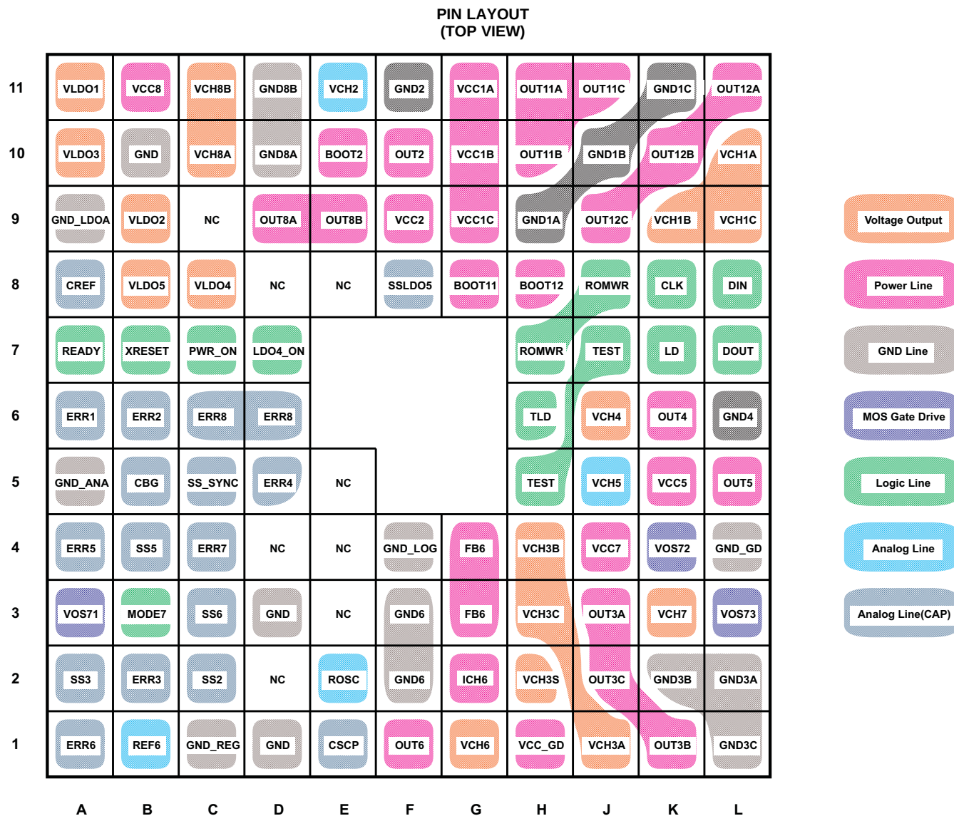
Figure 15. Pin Layout
